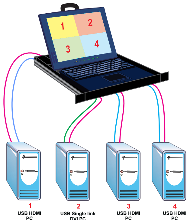
RACKMUX-D17HR-N-SUSBHD4
