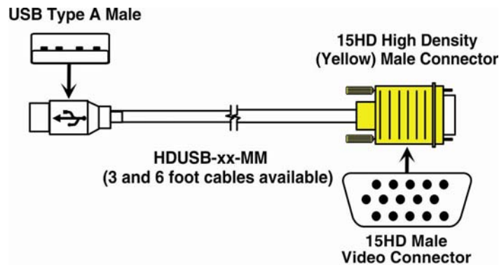
Figure 13- Cable for USB support only
