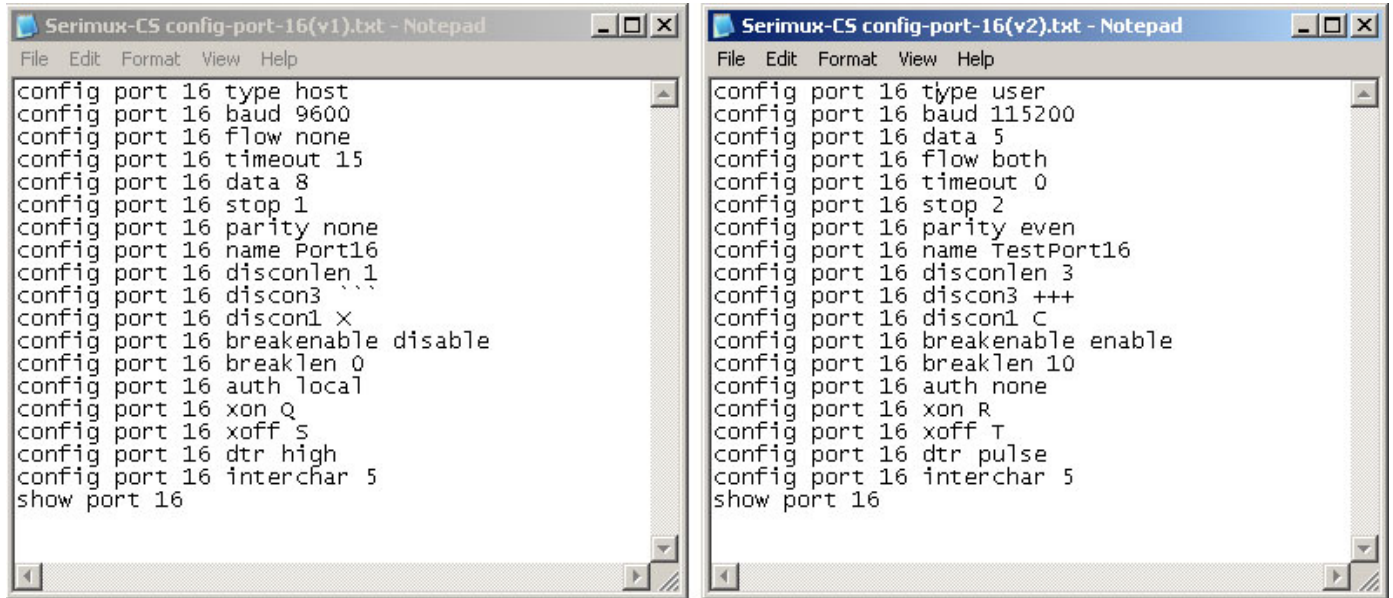
Figure 61- Sample txt files for configuring Port 16
