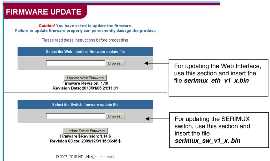
Figure 53- Firmware Update page
