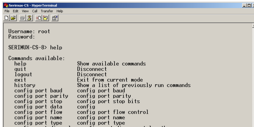
Figure 60- List of CLI commands
