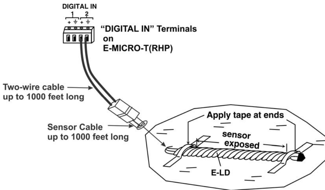
Figure 6- Secure liquid detection sensor with tape
