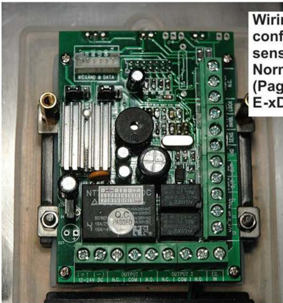
Circuit board inside E-ACK-VWT (Remove cover to view and wire)
