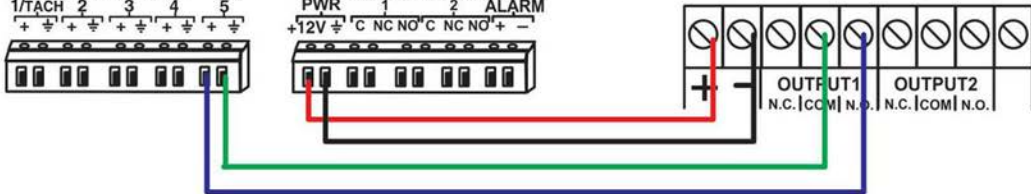
Terminals on E-5D
