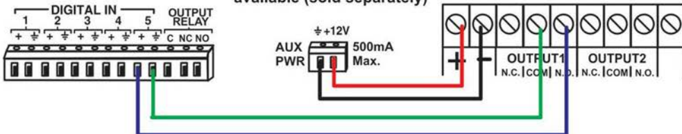
Terminals on E-ACK-VWT
